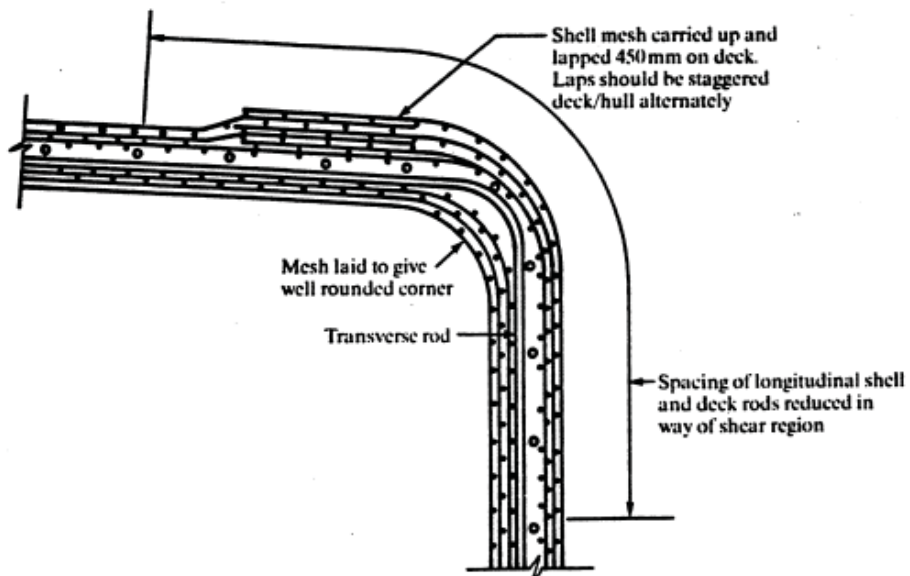
SECTION – DECK CORNER
