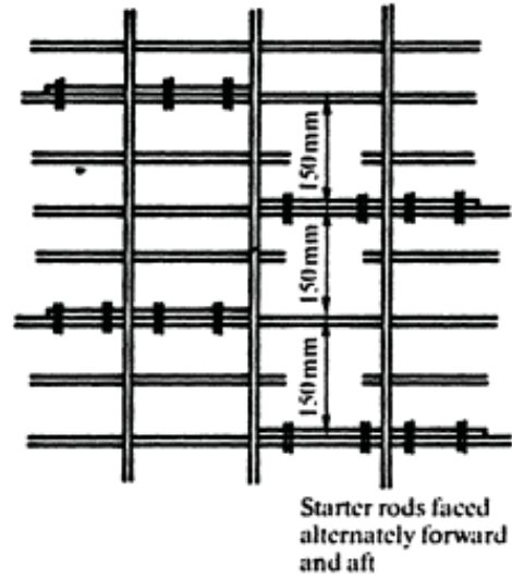
ELEVATION OF FRAME OR BULKHEAD-LOOKING OUTBOARD
