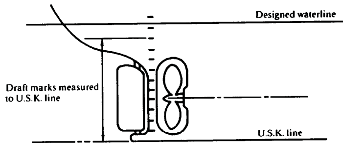
Figure 5 VESSEL WITH A STERN POST
