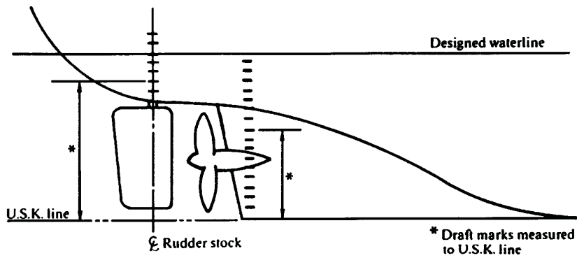
Figure 7 VESSEL WITH A SKEG AFT
