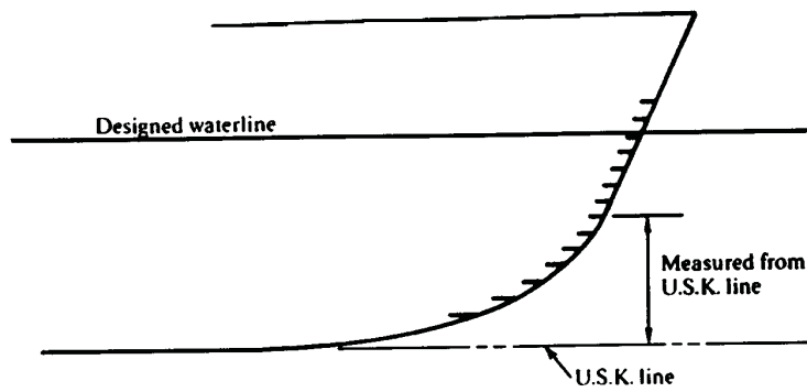
Figure 1 VESSEL WITH A RAKED STEM AND CUT-UP FORWARD
