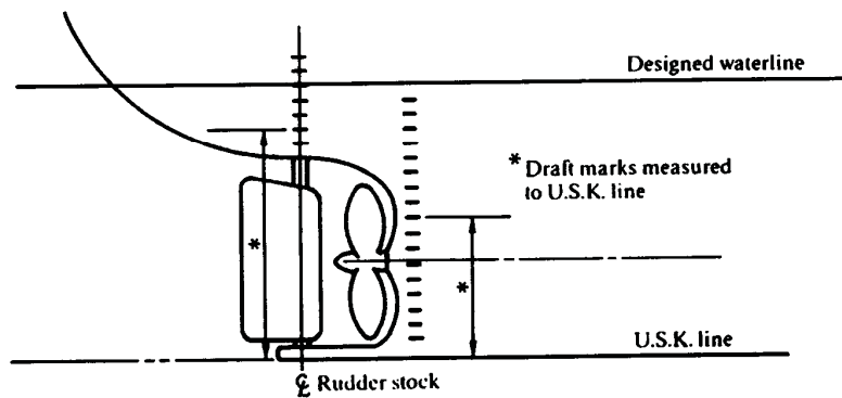
Figure 6 VESSEL WITHOUT A STERN POST
