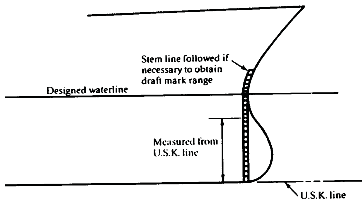
Figure 2 VESSEL WITH A BULBOUS BOW
