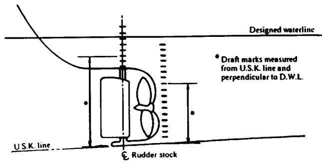
Figure 10 RAKED KEEL — VESSEL WITHOUT A STERN POST
