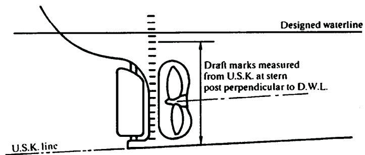
Figure 9 RAKED KEEL — VESSEL WITH A STERN POST
